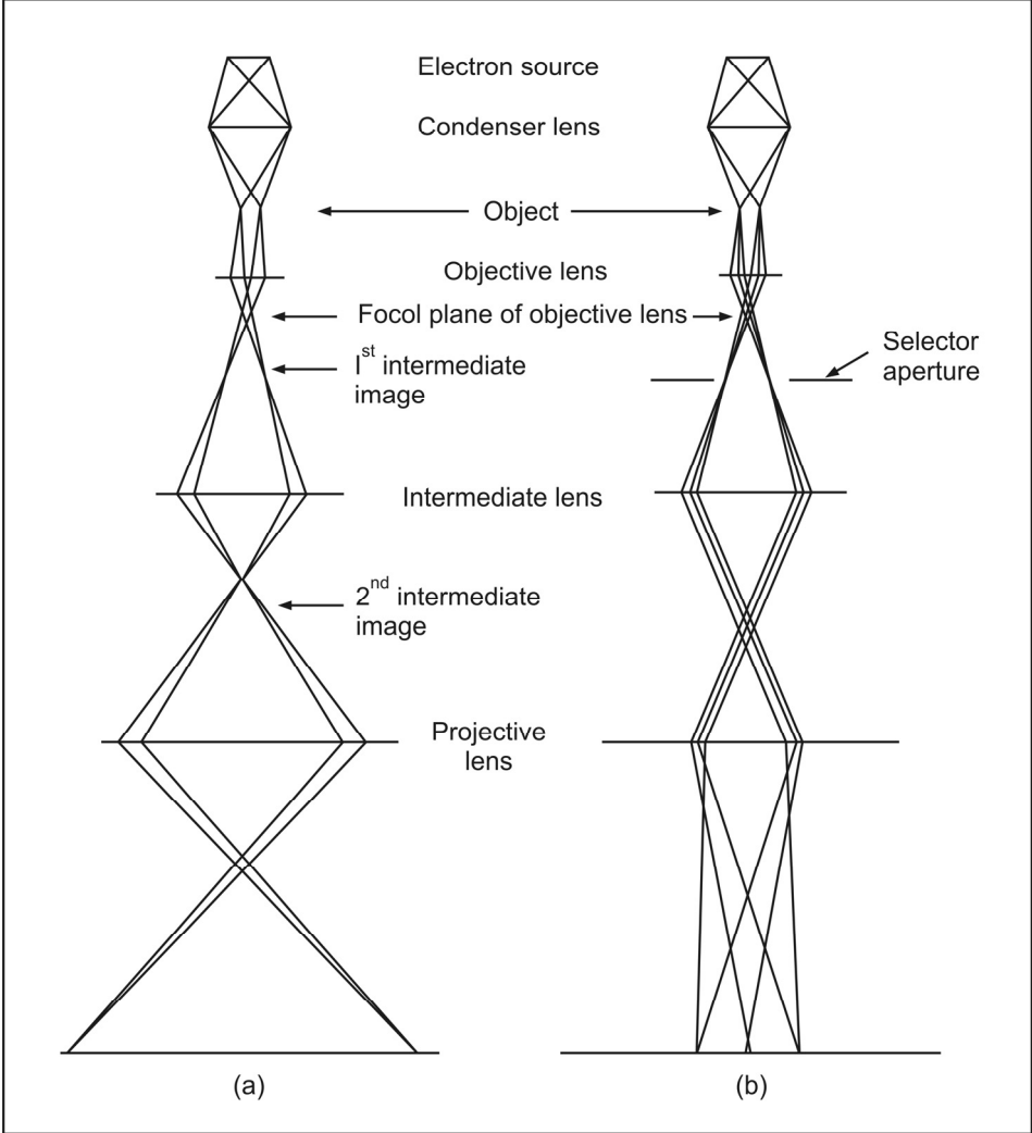
Fig. 1.11 The Electron Microscope (a) Cometrical optics representation of the TEM in imaging mode and (b) diffraction mode.
