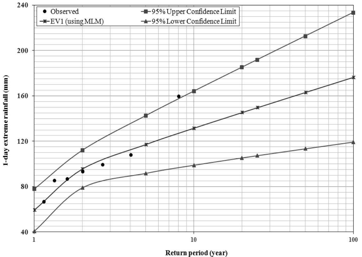
Fig. 1 Plots of recorded and estimated 1-day extreme rainfall with confidence limits
