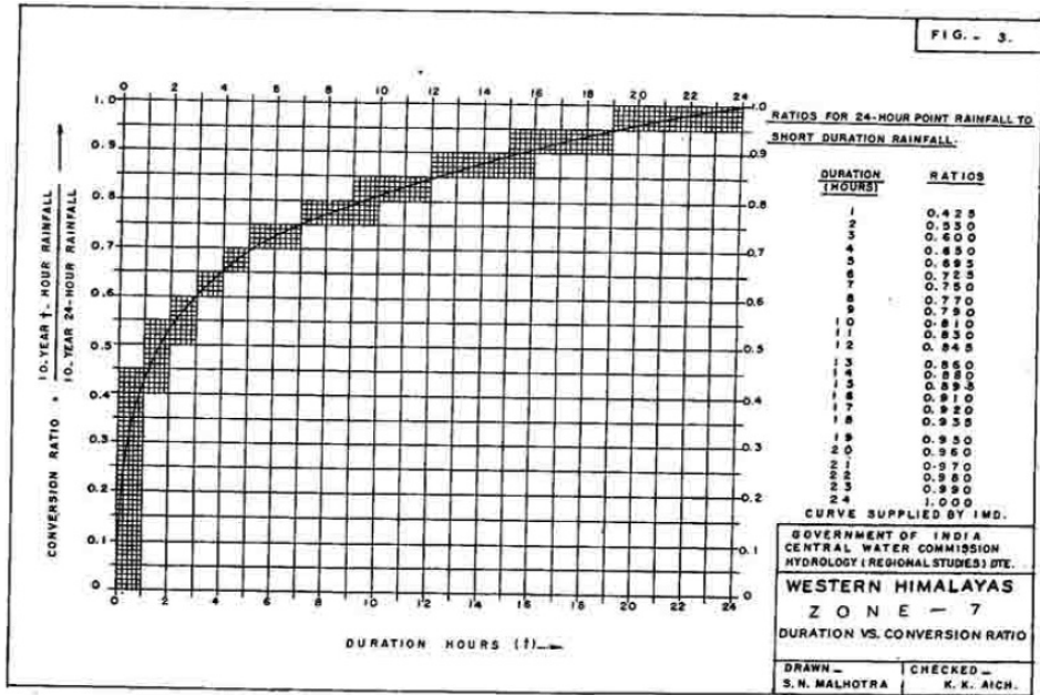
Fig. 2 Conversion factor for computation of distributed rainfall for shorter duration
